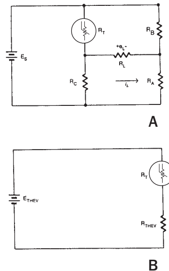
Figure 18: Wheatstone Bridge Circuits (Finite Load).
