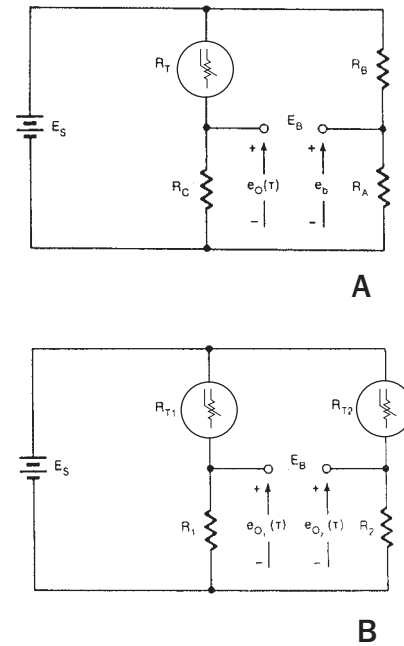
Figure 17: Wheatstone Bridge Circuits (Infinite Load).
