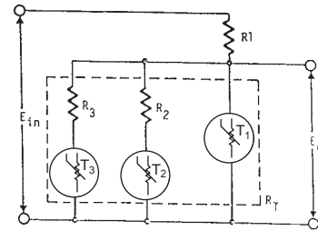
Figure 21: Multiple Thermistor Networks.
