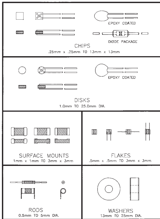
Figure 3: NTC Metallized surface contact type thermistor.
