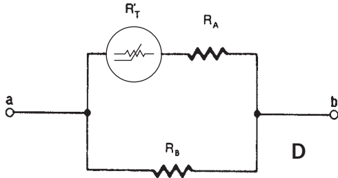
Figure 20: Linear Resistance Networks.
