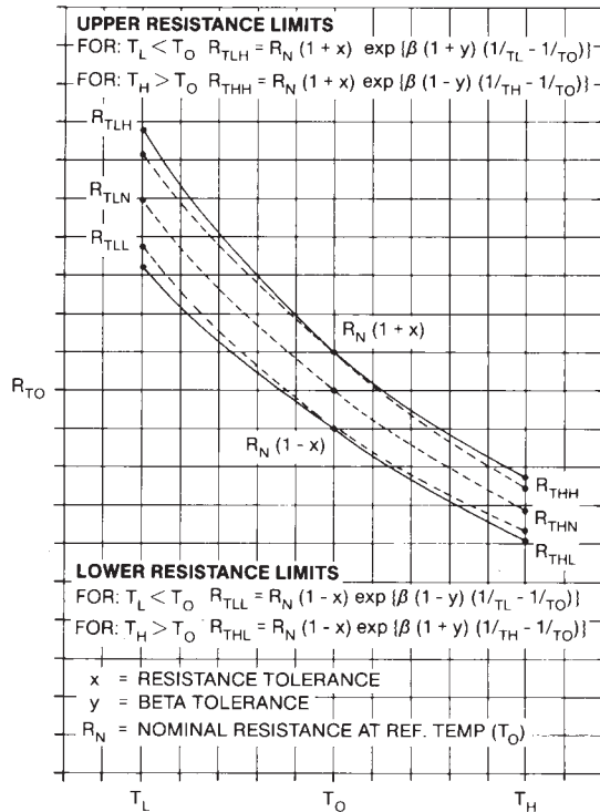
Figure 8: Effect of beta tolerance on Resistance Limits.
