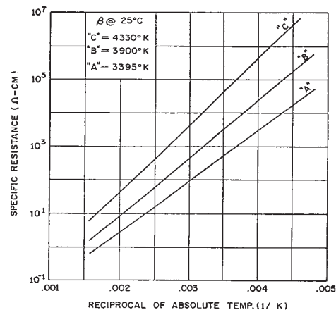
Figure 7: R-T Characteristics
