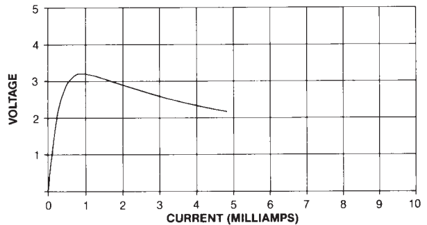
Figure 6: Typical Voltage-Current Characteristic (linear scale)
