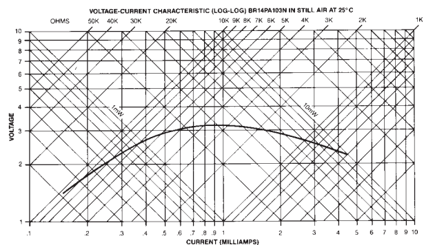
Figure 5: Typical Voltage-Current Characteristic (log-log scale)
