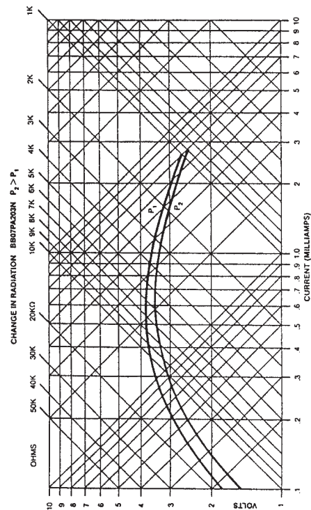
Figure 13: E-I Characteristics with changes in Absorbed Radiation.
