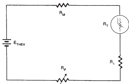
Figure 19: Ohmmeter Circuit.
