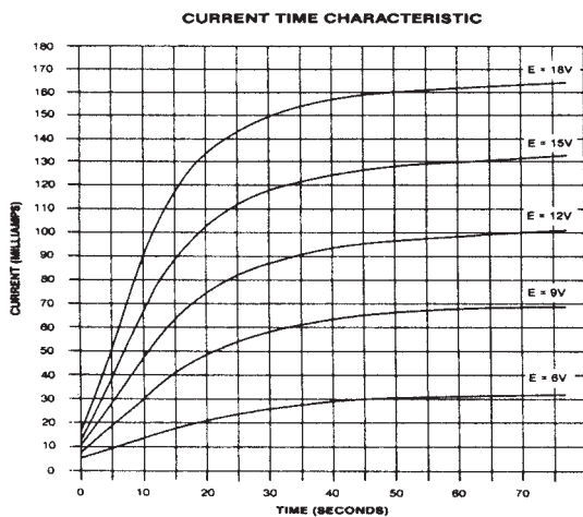
Figure 9: Example of current-time delay circuit.
