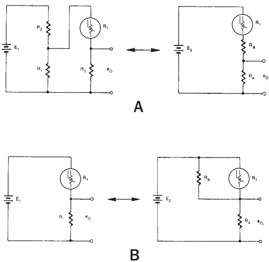
Figure 16: Modified Voltage Divider Circuits.
