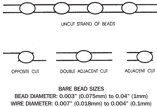
Figure 1: NTC Bead strands
